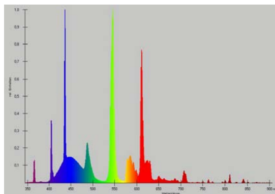
STUDIOLINE 55W/5600K
