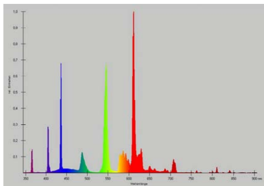
STUDIOLINE 55W/3200K
