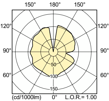
Light Distribution Diagram - MASTER CityWh CDO-TT Plus 70W/828 E27
