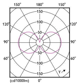
General uniform lighting - MAS LEDBulb D 4-60W E27 827 A60 CL G UE
