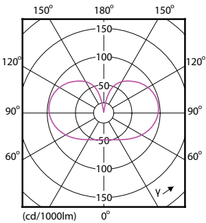
Light Distribution Diagram - MAS LEDBulb DT3.4-40W E27 CR195A60CL G
