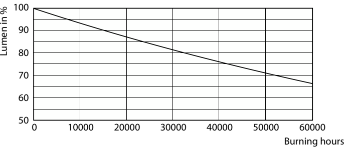
Lumen Maintenance Diagram - MAS LEDBulbND4-60W E27 827 A60 CL G UE
