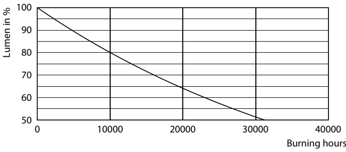
Lumen Maintenance Diagram - CorePro LEDbulb ND 10-75W A60 E27 940
