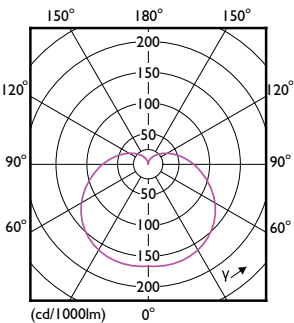
Light Distribution Diagram - CorePro LEDbulb ND 11-75W A60 E27 927
