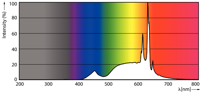
Spectral Power Distribution Colour - CorePro LEDbulb ND 11-75W A60 E27 927
