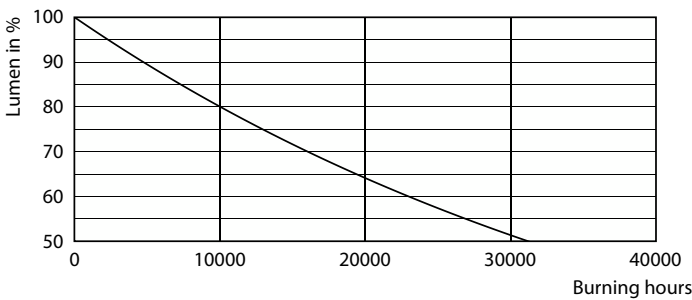
Lumen Maintenance Diagram - CorePro LEDbulb ND 7.5-60W A60 E27 940
