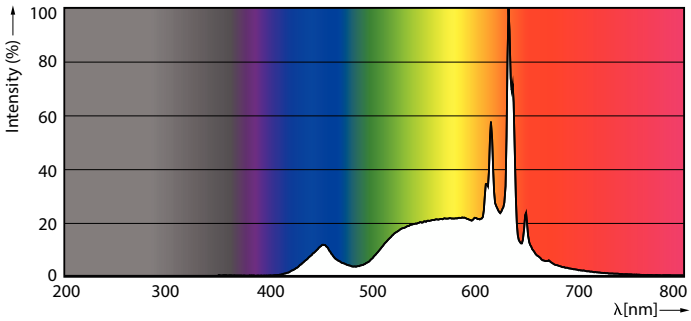
Spectral Power Distribution Colour - CoreProLEDbulb ND 4.9-40W A60 E27 927
