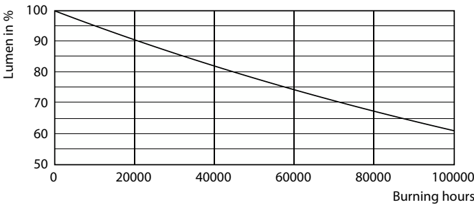
Lumen Maintenance Diagram - MAS LED SON-T EM 10.8Klm 65W 727 E40
