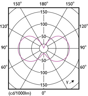
Light Distribution Diagram - MAS LEDLusterDT5.9-60W E27 927 P45CL G
