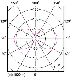
LED Bulb A67 E27 ND Clear
