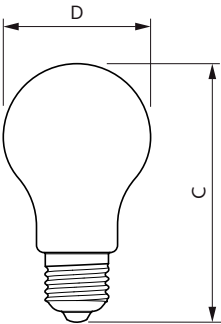
CorePro LEDBulbND10.5-100W E27A60 827CLG
