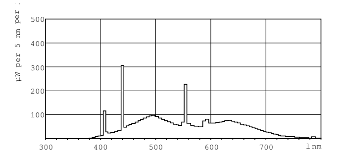
LDPB_TL-D9HCR_965-Spectral power distribution B/W
