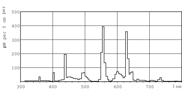
LDPB_TL5HO8SE_840-Spectral power distribution B/W
